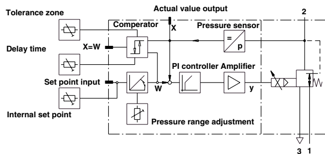
Block diagram (enlarged)
