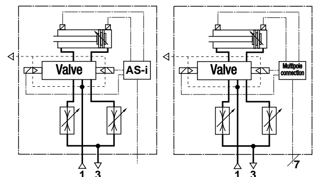
SMART-Cylinder with AS-Interface Bus System
