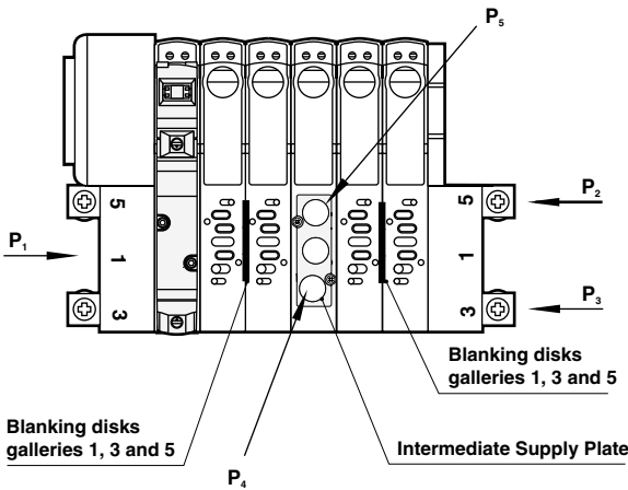
Five pressure
