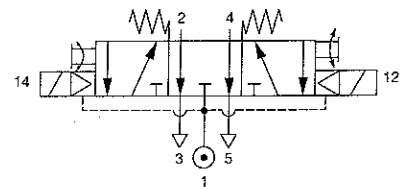
Model Number: M/1744/8123 Type: 5/3 Fully sealed mid-position Integral Pilot Supply
