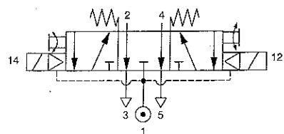
Model Number: M/1754/8123 Type: 5/3 Supply sealed mid-position Integral Pilot Supply
