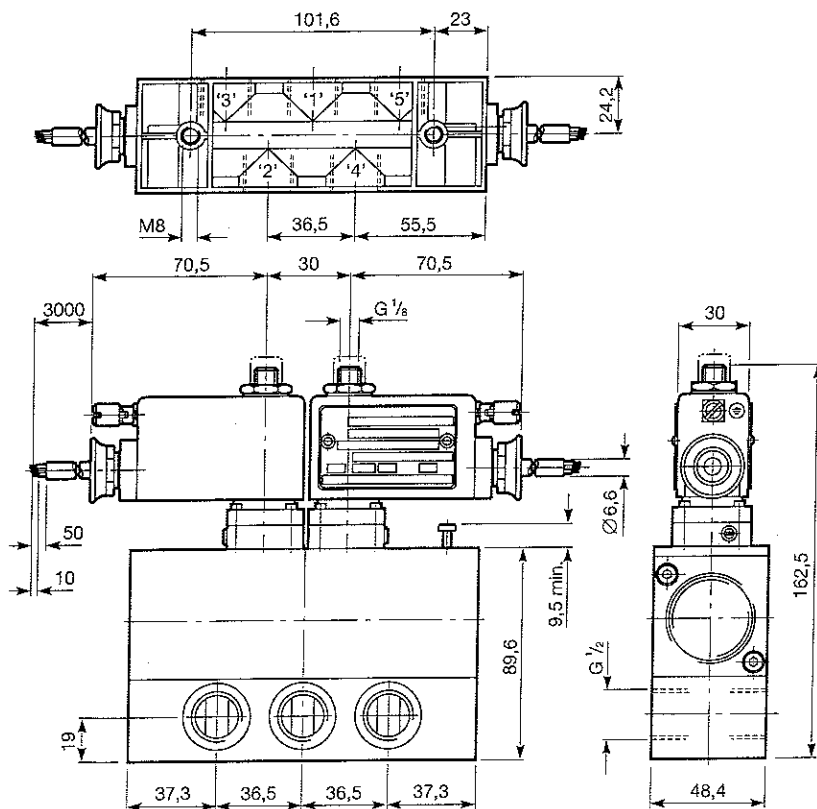
Model Number: M/1754/8123 Type: 5/3 Supply sealed mid-position Integral Pilot Supply
