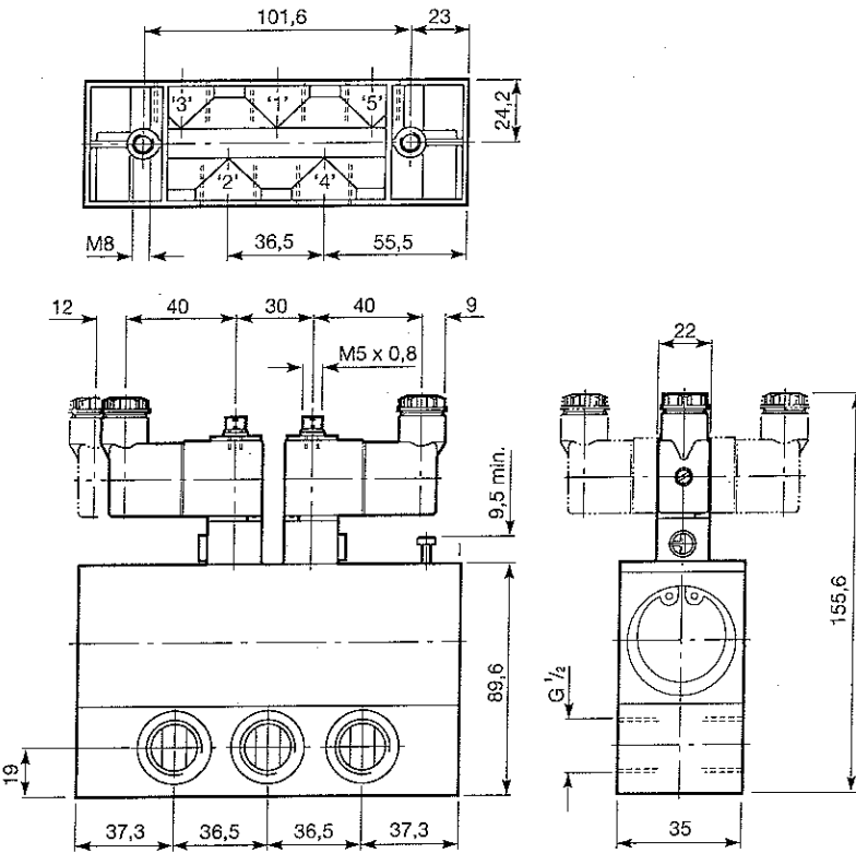
Model Number: M/1774/6123 Type: 5/3 Supply sealed mid-position Integral Pilot Supply
